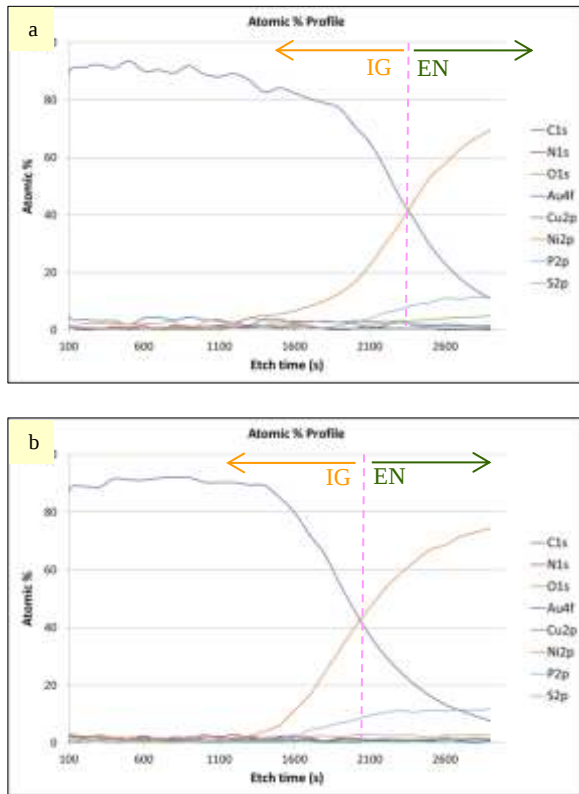
Figure 5: Atomic % depth profile of IG layer to ENIG interface for the as-plated sample of (a) the fresh CN free immersion gold bath and (b) aged CN-free immersion gold bath with 700ppm Ni and 6ppm Cu.
