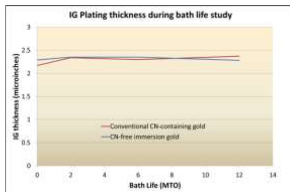
Figure 1: Comparison of IG plating thickness for the CN-free immersion gold bath (45°C, 11 min) and Conventional CN-containing gold bath (84°C, 8 min) as a function of bath life.
