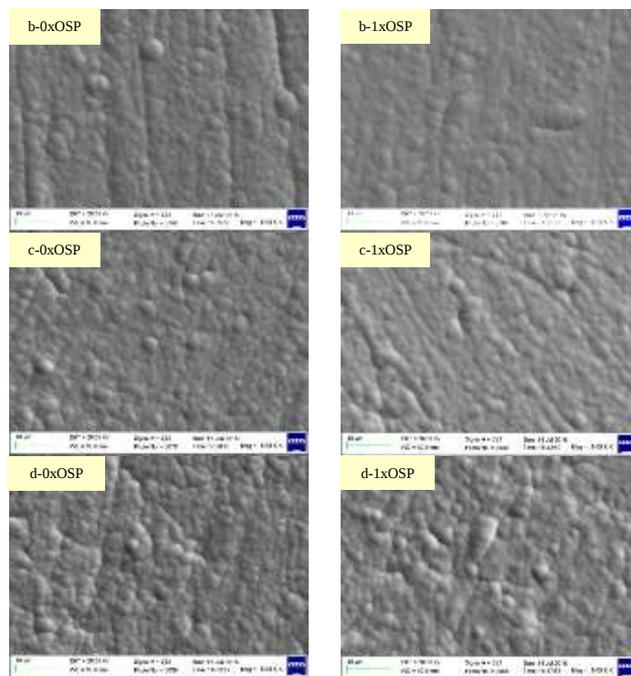
Figure 3: SEM images of EN surface for as-plated (0 x OSP) and after OSP simulation (1 x OSP; copper etch 0.75μm) of ENIG after gold stripping; (a) 0 MTO (b) 2 MTO (c) 6 MTO and (d) 12 MTO.
