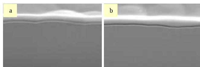
Figure 4: Cross section FIB-SEM images of ENIG deposit for (a) fresh bath and (b) aged bath from Cyanide-free immersion gold chemistry.
