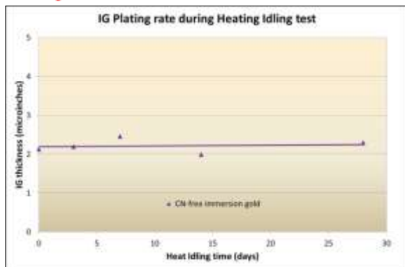
Figure 2: IG plating thickness for the CN-free immersion gold bath (45°C, 11 min) as a function of time of heat idling at 50°C.
