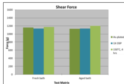
(a) Shear Force and Failure mode of the ENIG deposit of Cyanide-free immersion gold
