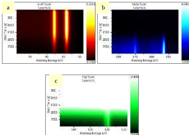
Figure 6: Elemental scan during depth profile of IG layer to ENIG interface (a) Au scan (b) Ni scan and (c) P scan of aged CN-free immersion gold bath with 700ppm Ni and 6ppm Cu.
