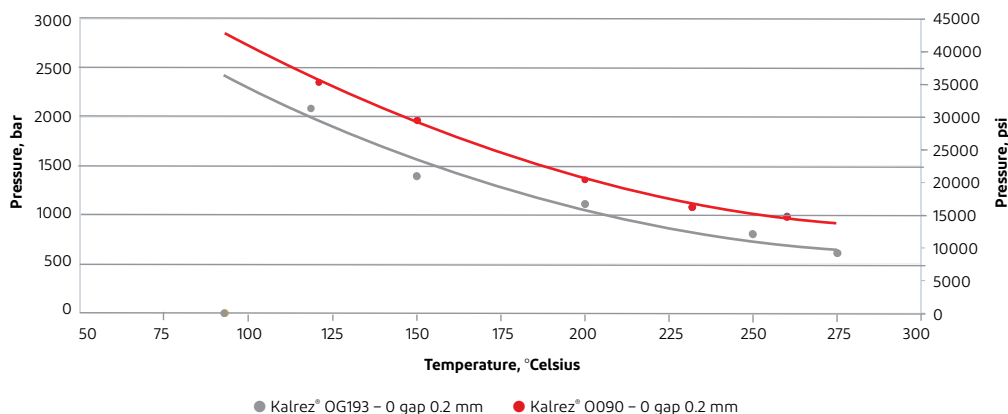
Extrusion resistance of Kalrez® OG193 versus Kalrez® 0090
