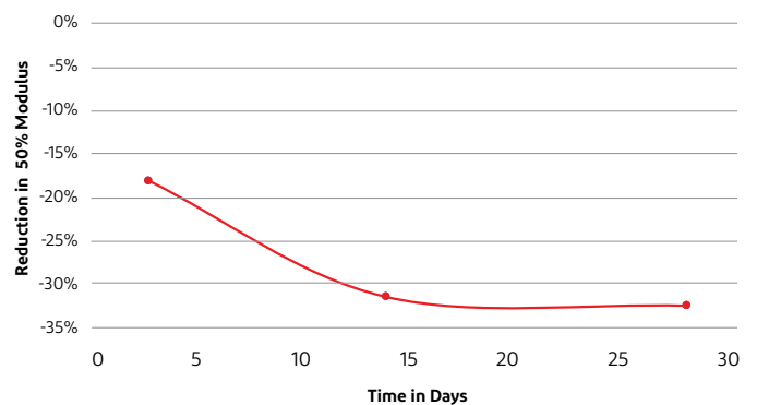
Kalrez® 0090 Exposure to 35% H 2 S, 35% CO 2 at 220 °C
