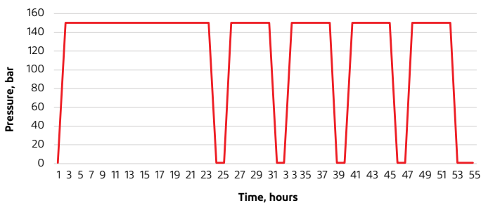
Kalrez® OG193 RGD cycling test: 150 °C - 150 bars - 127 bar/min
