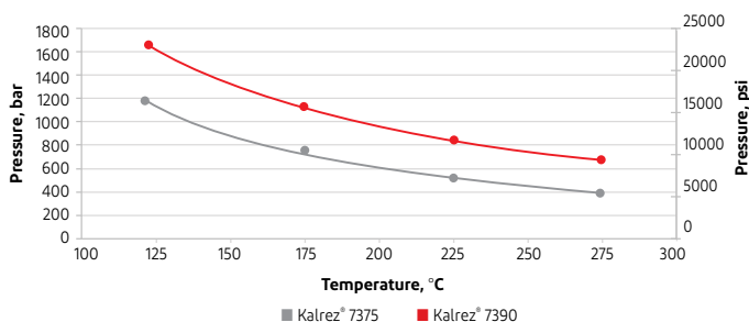
Extrusion resistance of Kalrez® 7375 versus 7390
