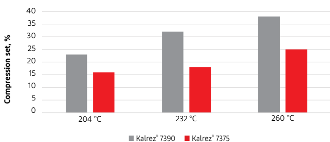
Compression Set, % (with 25% squeeze) of Kalrez® 7390 and Kalrez® 7375 at various temperatures at 672 hours
