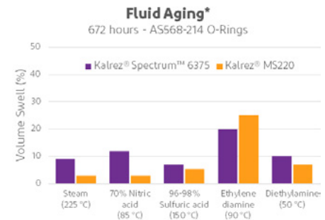
Kalrez® MS220 vs Kalrez® Spectrum 6375 Chemical resistance
